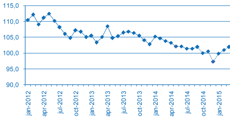
Fig. 46. Employment (million people)
